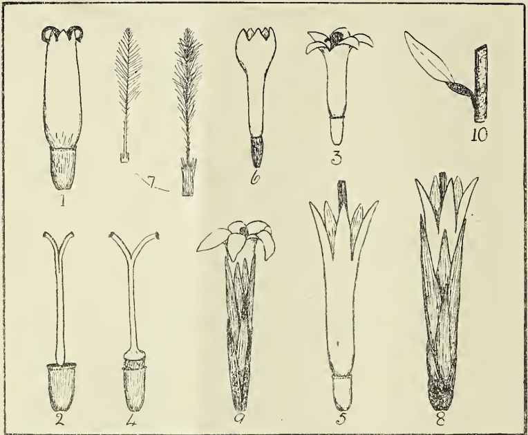
FIG. 1. Stoebe incana . Flower with pappus removed, ready for pollination \times 12 .
